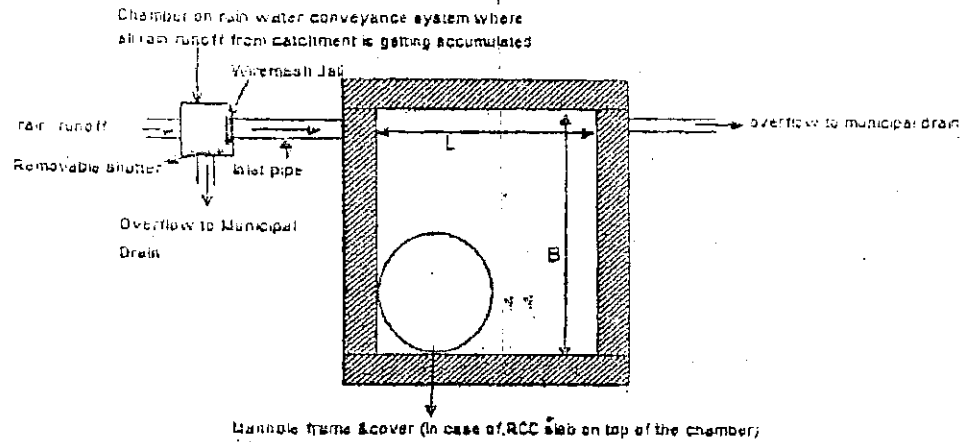
Fig. 1 : Rectangular Recharge Chambers for RWH
